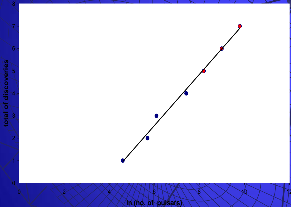
Pulsar-discoveries
